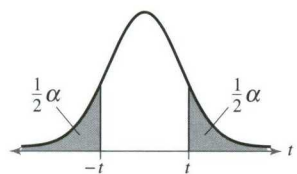
Two-tailed test
