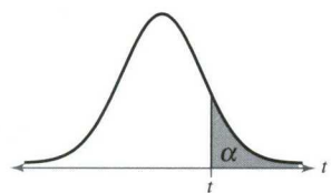
Right-tailed test
