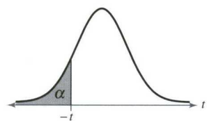
Left-tailed test
